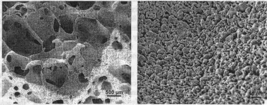
Fig. 2 Porous calcium phosphate scaffold material (Ca/P=1.45), after calcination at 1000°C; 35±2 MPa compressive strength: (left) interconnected macropores, (right) magnified view of the same sample, which thus reveals the microporous nature of those dense-looking struts/walls
